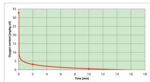
Fig. 4: Oxygen content of linseed oil during ISO-MIX treatment
