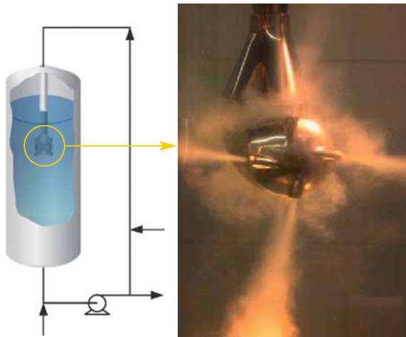
Fig. 2: Rotary jet head
